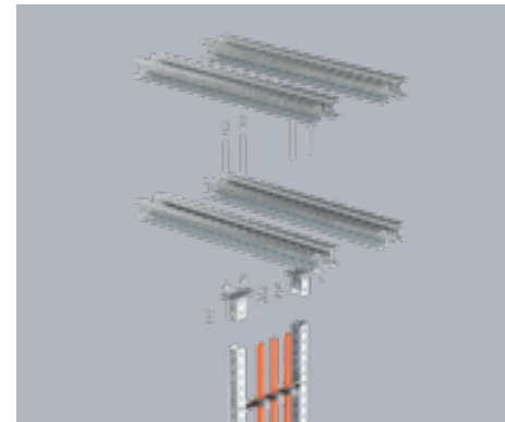
Direkte Montage der Steigeleiter Typ SLS80C40F ... an Massivwand Direct mounting of the vertical ladder type SLS80C40F ... on solid wall
